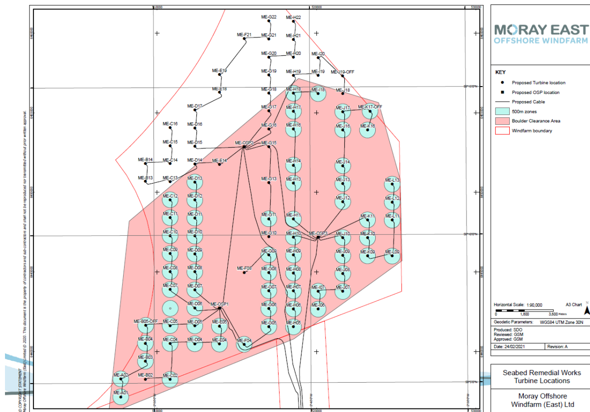
Figure2. Clearance Works Locations
