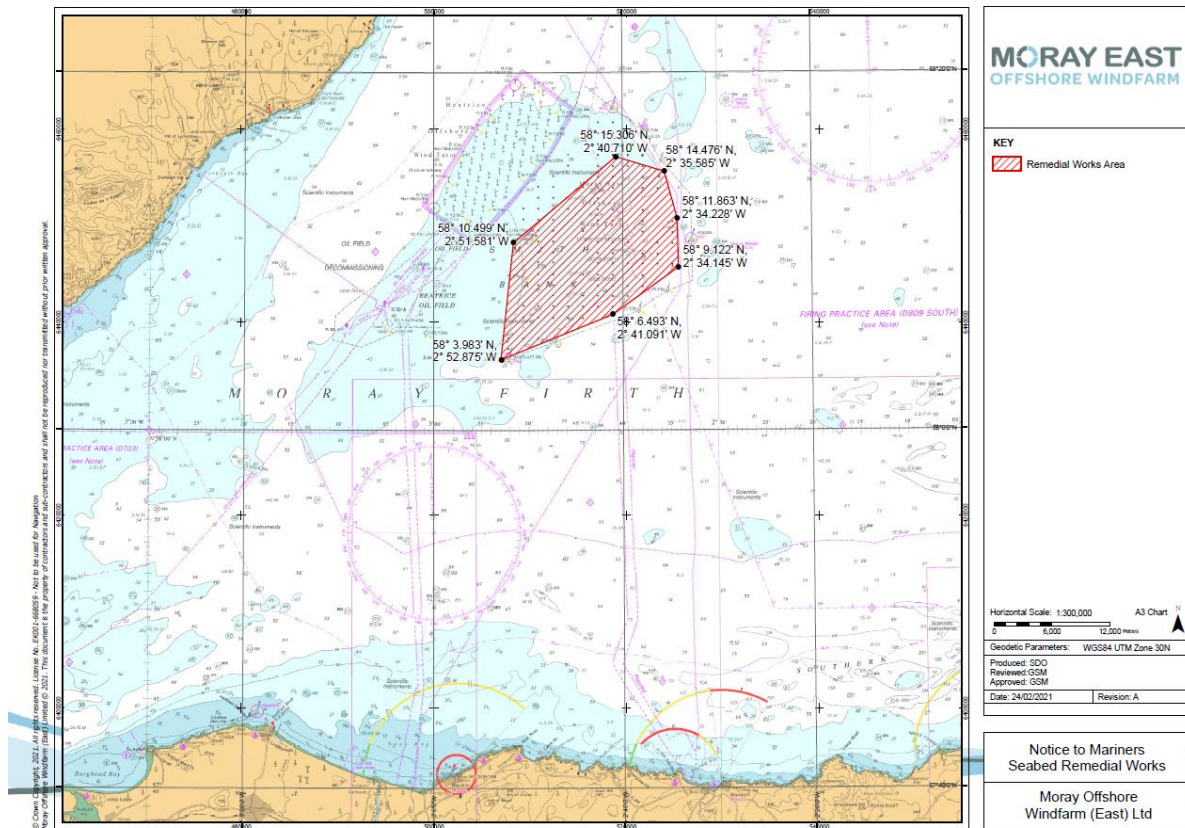
Figure 1. Remedial Works area
