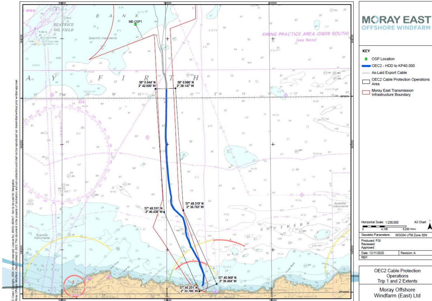
Figure 2. Bounded Cable Protection Area
