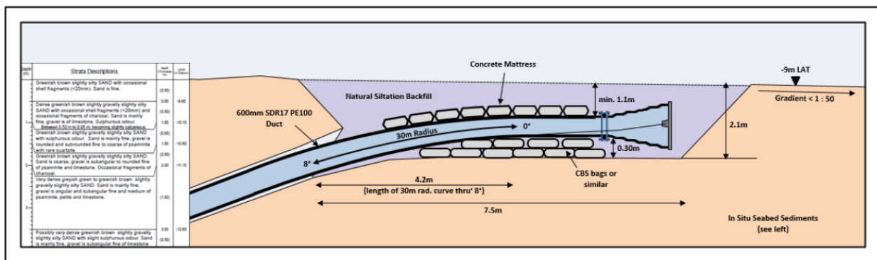
Figure 7 – As left detail of ducts in seabed
