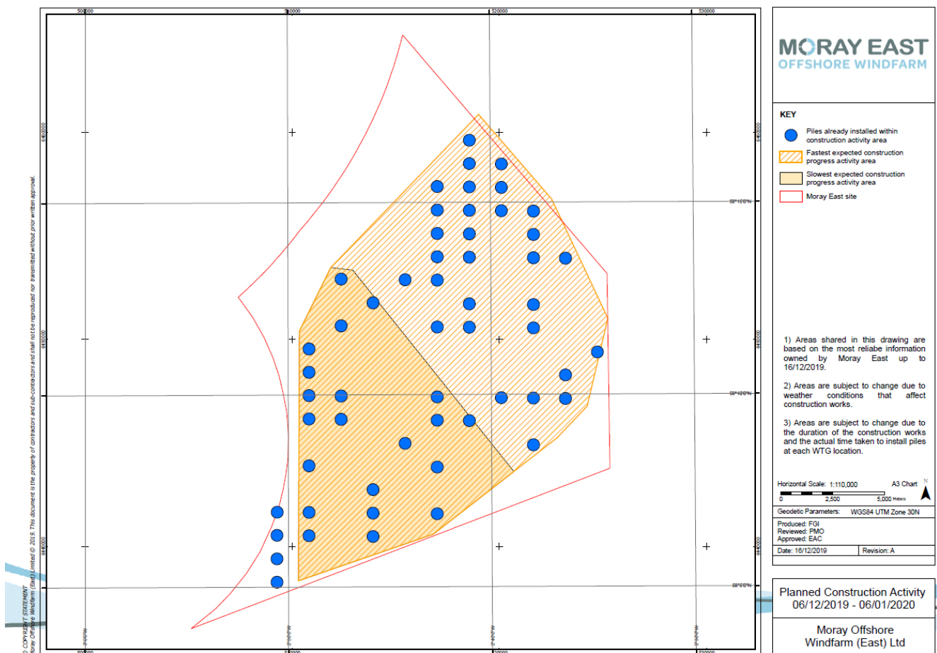
Figure 4 – Piling activity area expected for between 16th December and 13th January 2020
