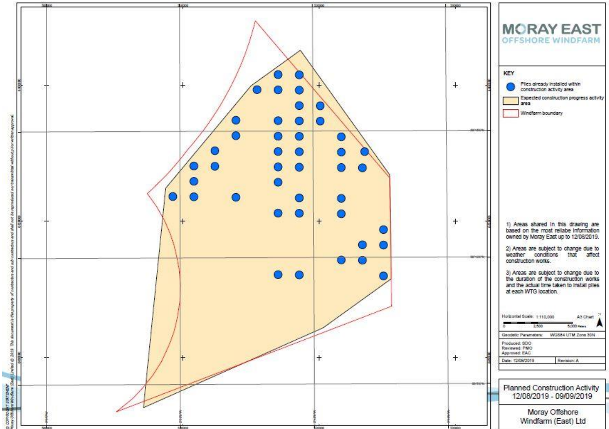
Figure 5 – Piling activity area expected for between 12 th August and 9 th September 2019
