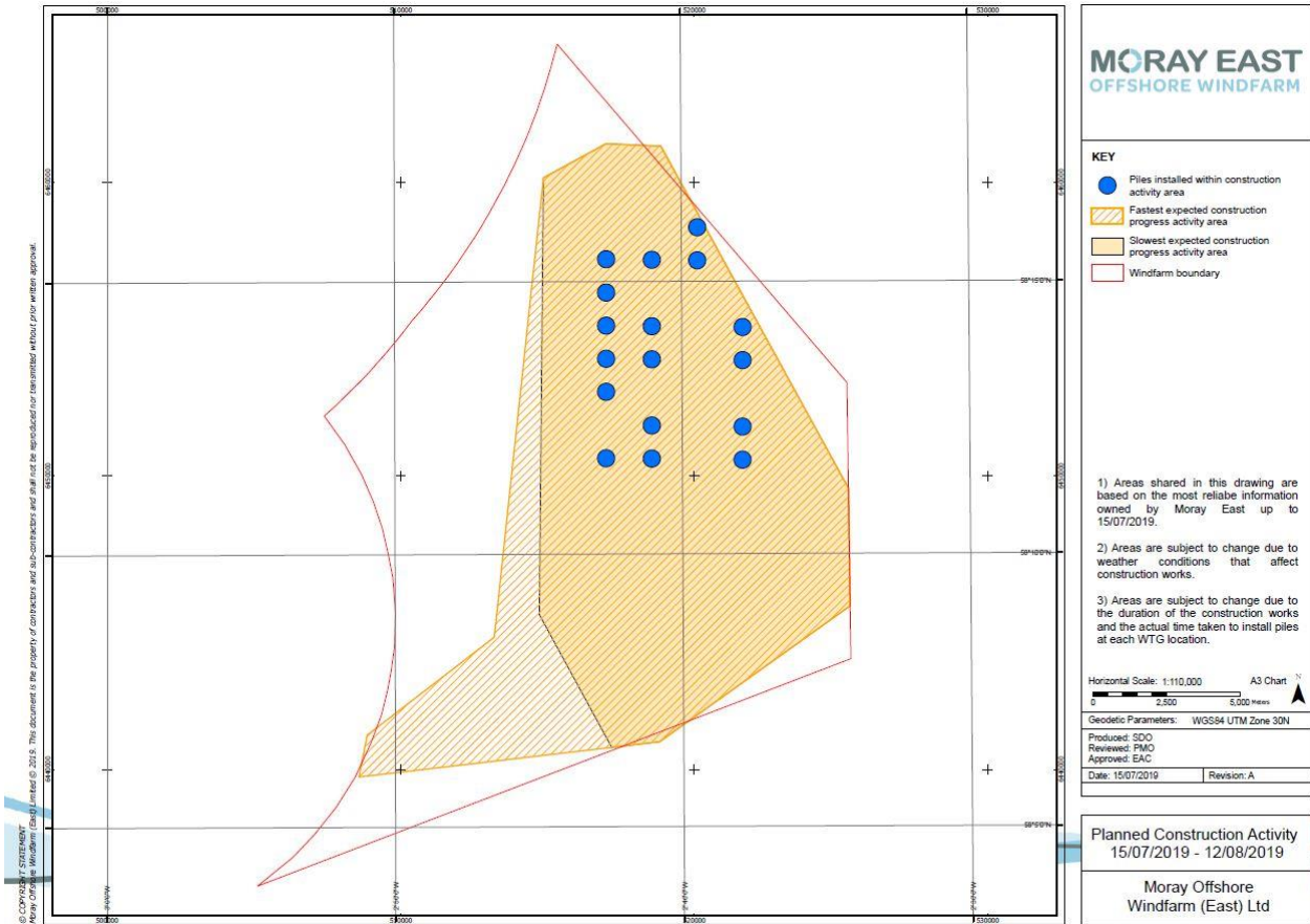
Figure 5 – Piling activity area expected for between 15 st July and 12 th August 2019
