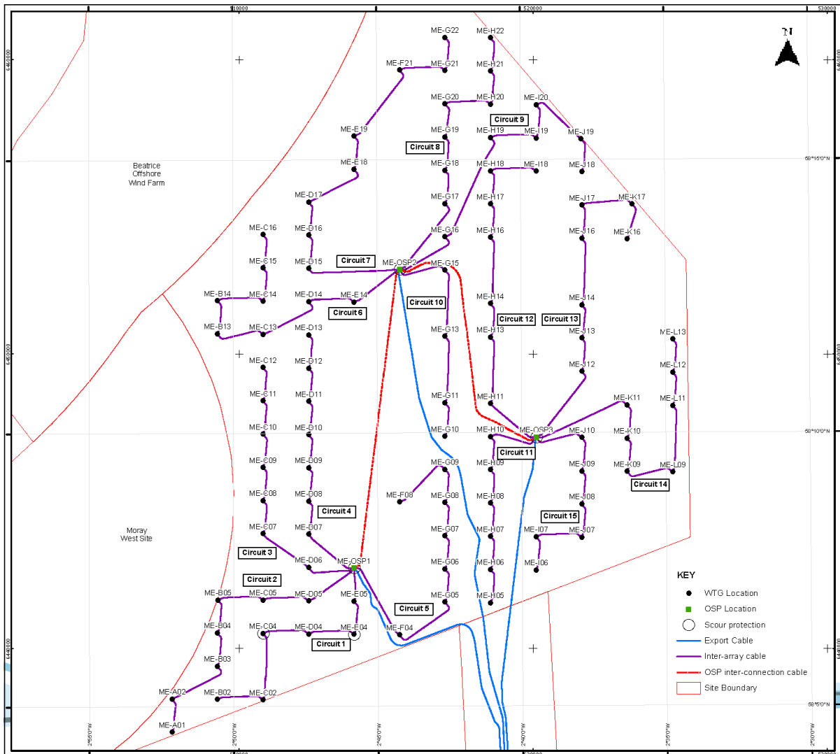
Figure 1 Moray East Site Layout
