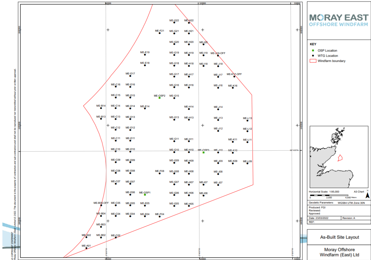
Figure 1. Moray East site layout
